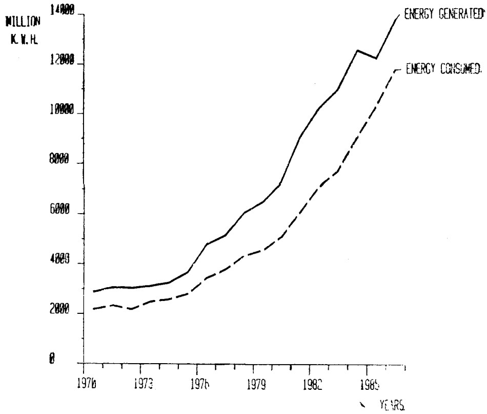
ENERGY GENERATED & CONSUMED 1970-71 TO 1986-87
