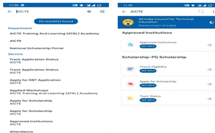
Fig 5.1.1: UMANG Application
